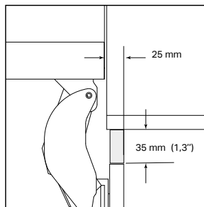
115° DEUROPENING
