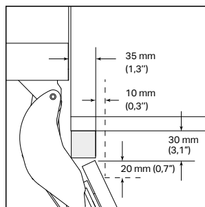
115° DEUOPENING
