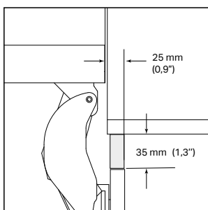
90° DEUOPENING
