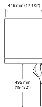
DEUROPENING 90°
