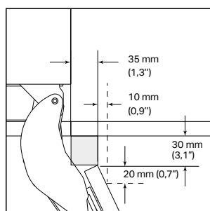
115° DEUROPENING
