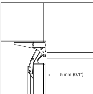
90° DEUROPENING
