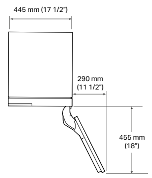
DEUROPENING 115°
