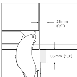
90° DEUROPENING
