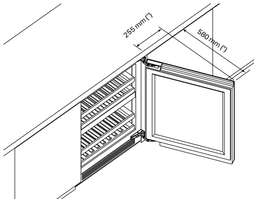
115° DEUROPENING
